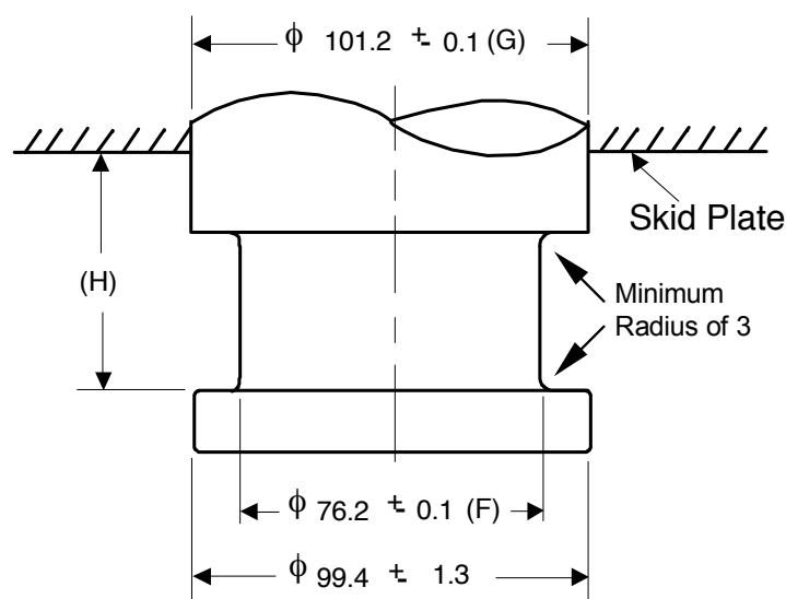
Dimensions of a 75 mm kingpin
